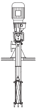
BE RANGE SEMI-SUBMERSIBLE VARIANT O
