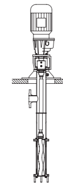
BE RANGE SEMI-SUBMERSIBLE VARIANT U
