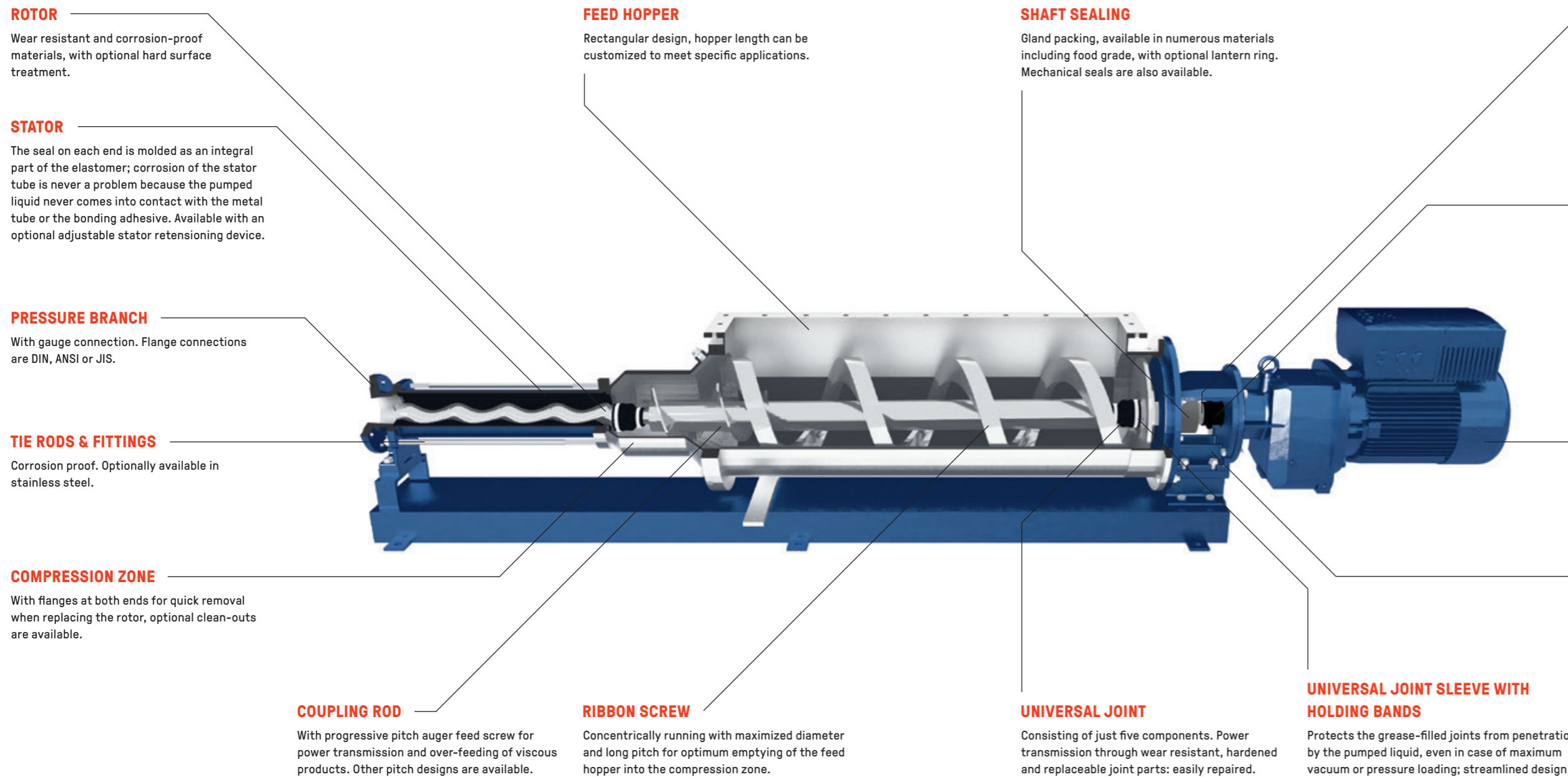
Picture: BTHE range pump
